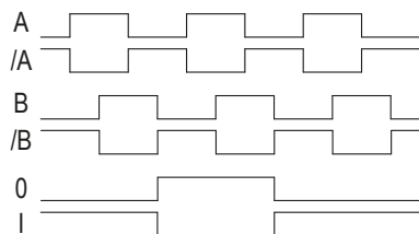
Fig. 9: Wave form
